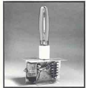
BALLAST KIT ASSEMBLY
